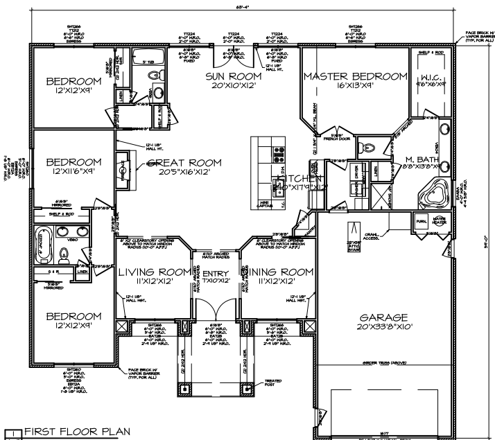
1 FIRST FLOOR PLAN A-3
