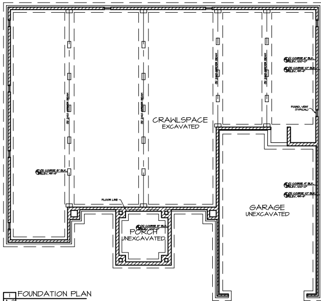
1 FOUNDATION PLAN A-2
